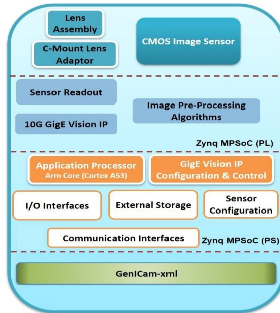
Fig. 1. iViS-10GigE architecture
