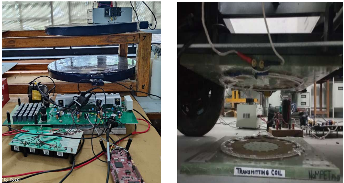
Fig.2. Wireless charger system
